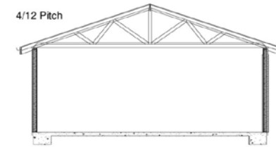
Cross Section
