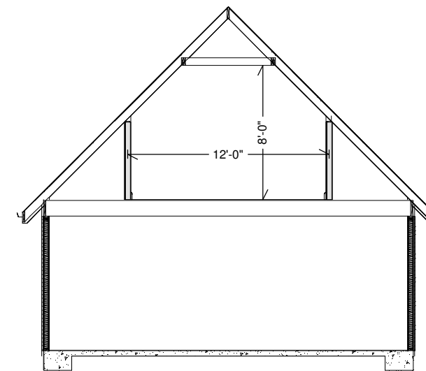
Cross Section
