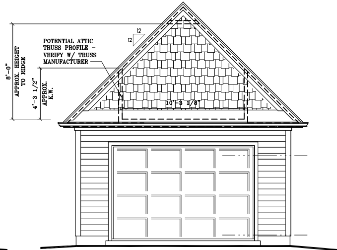
Front Elevation 12:12 Roof Pitch
