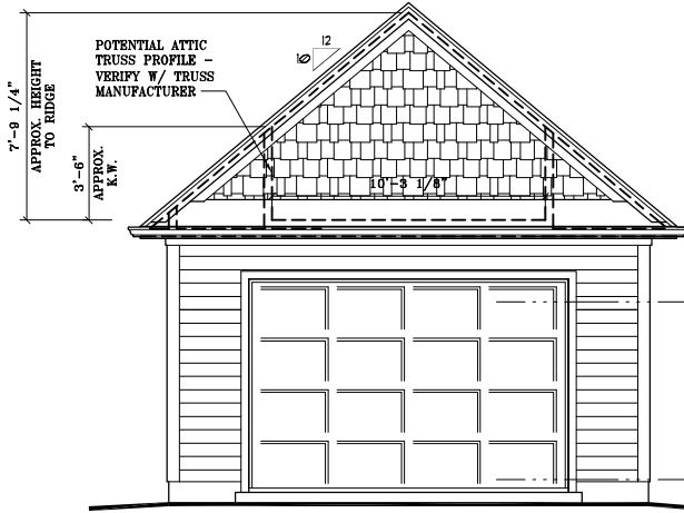
Front Elevation 10:12 Roof Pitch
